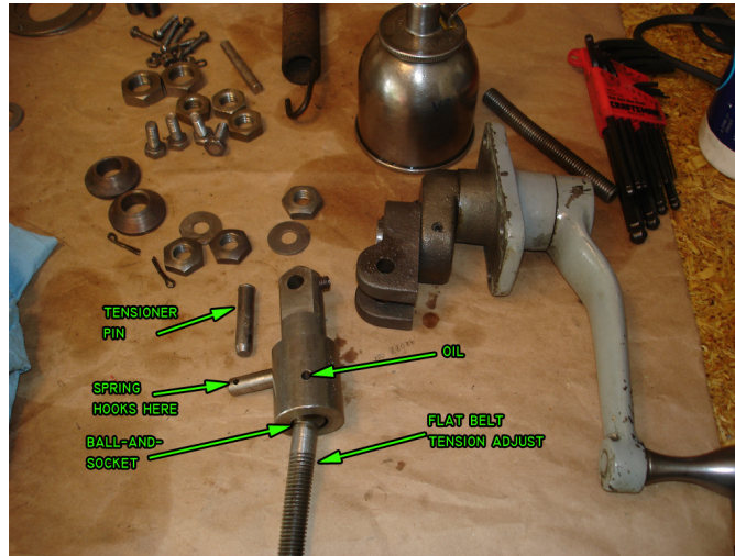
Figure 25: The assembled tensioner to show functionality.
