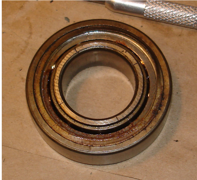
Figure 16: Original countershaft bearing with shield removed.
