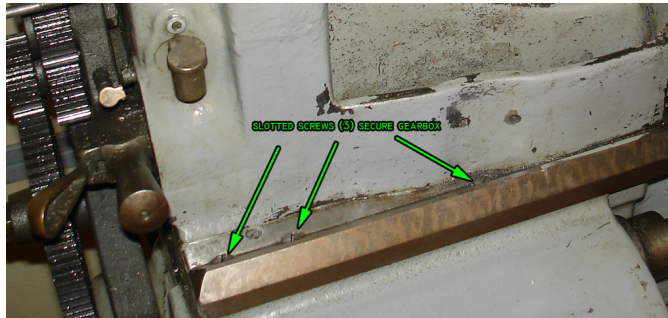
Figure 123: Screws that secure the gearbox to the bed.
