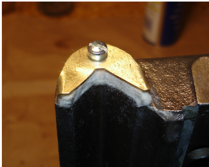
Figure 190: New saddle felt.
