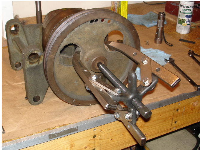
Figure 11: Pulling the vee-belt pulley using a 7-ton OTC brand 2/3-jaw puller.
