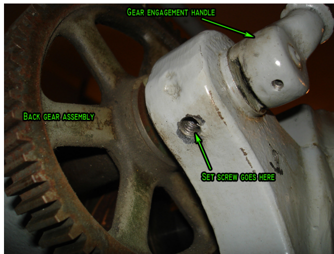
Figure 33: Set screw below the engagement handle that retains the back gear shaft.
