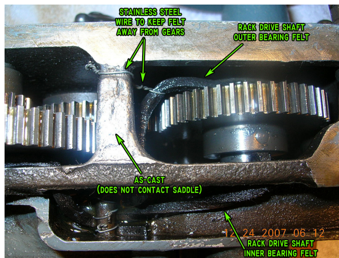
Figure 171: A heavy 10 apron showing different upper felt routing.
