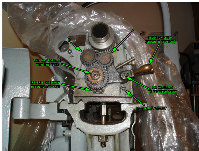
Figure 62: Reversing gear train prior to removal.
