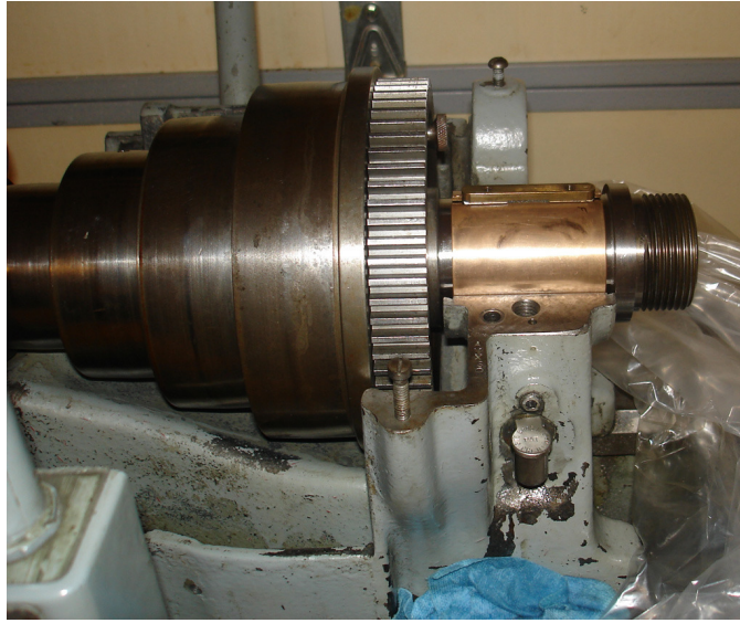
Figure 60: Reinstalled headstock spindle showing front bearing
