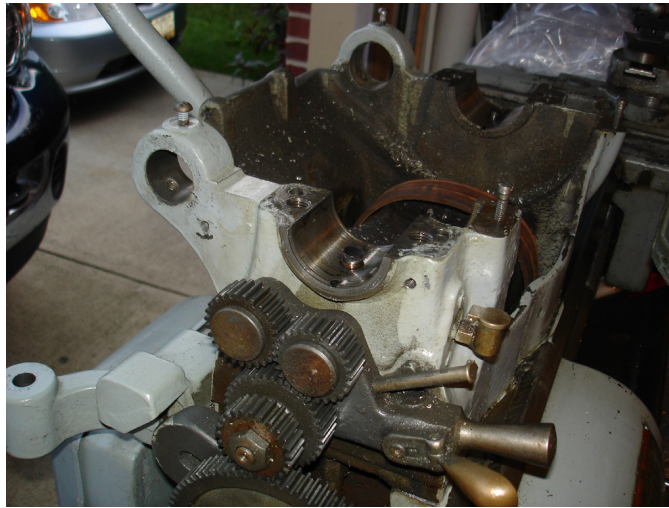
Figure 72: Overview of headstock casting with spindle removed.
