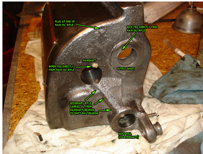
Figure 139: Side of gearbox showing lubrication points.
