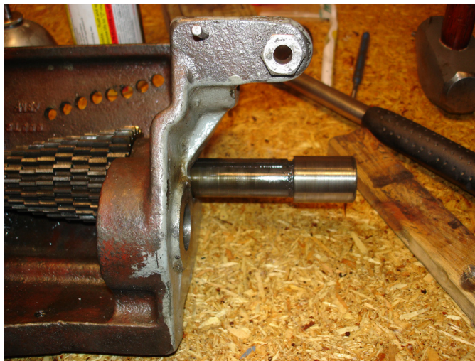
Figure 134: Mainshaft being removed.
