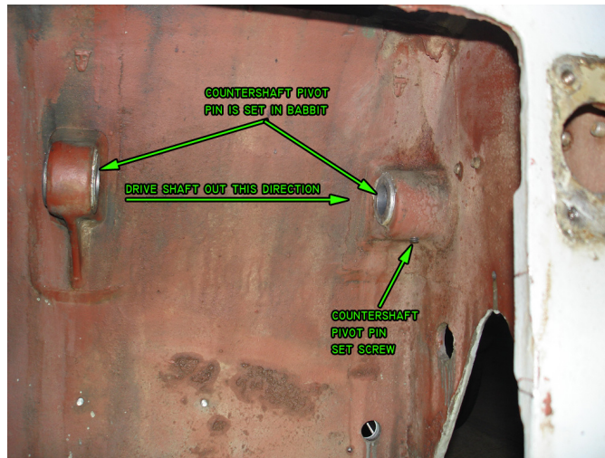
Figure 5: Showing location of countershaft pivot set screw.
