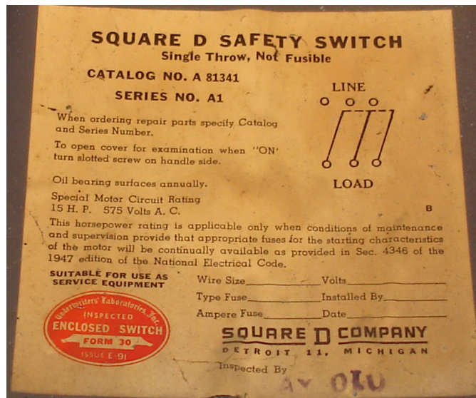
Figure 98: Notice page inside safety switch.
