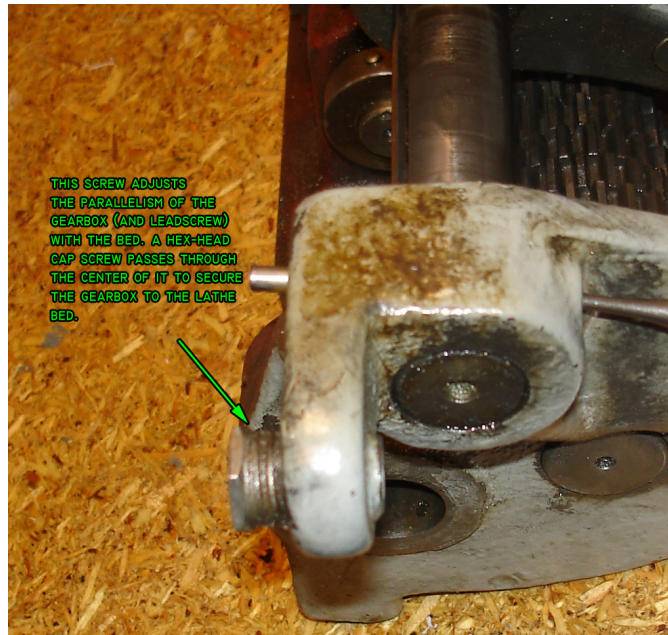
Figure 125: Gearbox parallelism adjuster.
