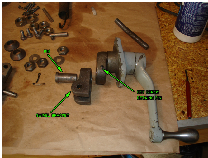
Figure 24: Tensioner assembly.
