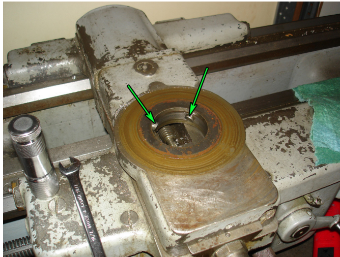
Figure 103: Carriage with compound rest removed.
