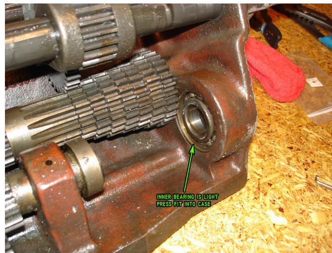
Figure 128: View of inner leadscrew bearing with leadscrew removed.
