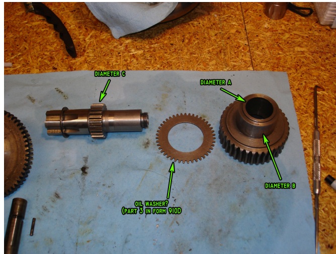
Figure 162: Clutch parts showing unusual gear.
