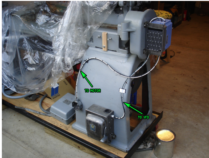
Figure 91: Installed safety switch.
