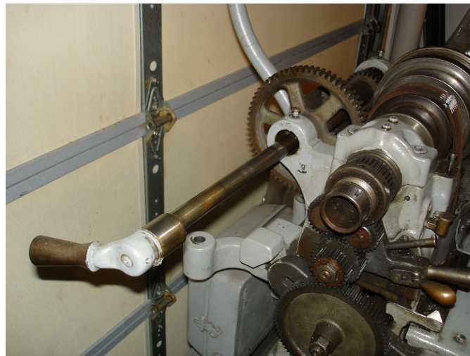
Figure 35: Removing the back gear spindle.
