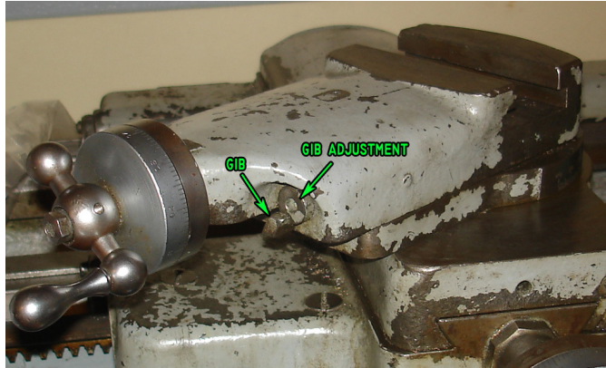
Figure 108: Compound rest gib adjuster.
