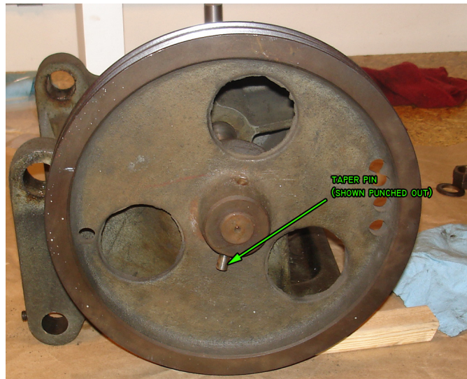
Figure 10: Vee-belt pulley being removed.
