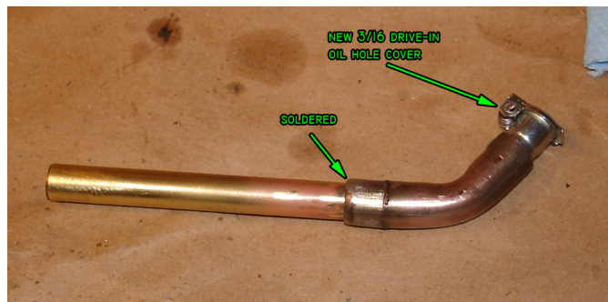
Figure 182: Repaired apron oiler.
