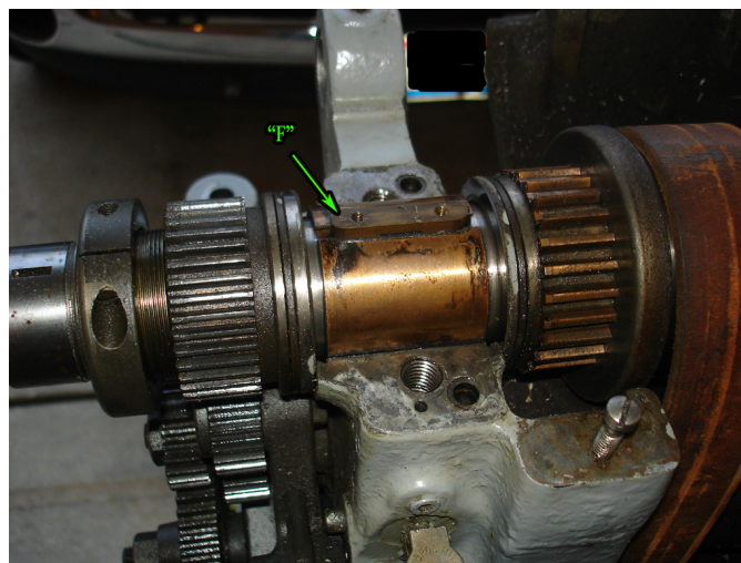
Figure 40: Rear bearing cap removed. Notice the "F" indicates this expander is in the wrong orientation.
