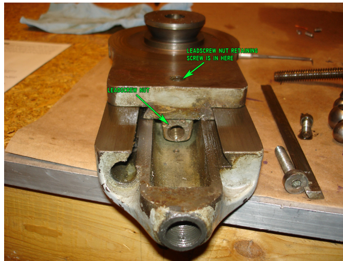
Figure 110: Location of compound rest leadscrew nut retaining screw.
