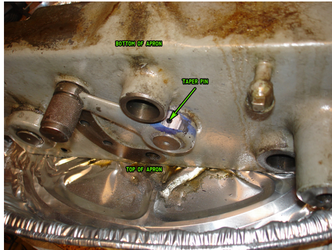
Figure 166: Drive selector taper pin.
