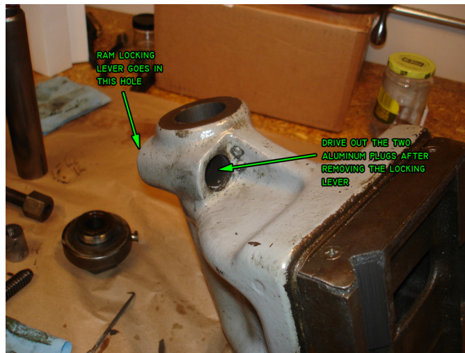
Figure 197: Tailstock ram locking mechanism removed.
