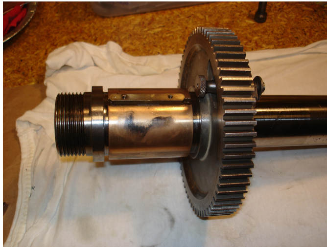
Figure 58: Bull gear installed.
