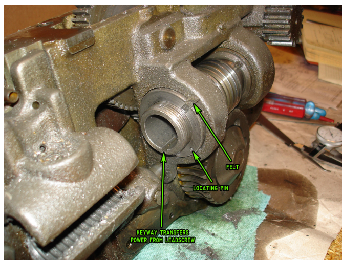
Figure 155: Worm drive end bushings.
