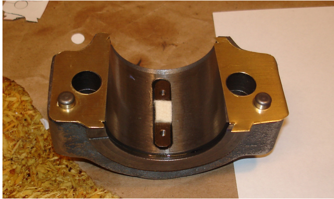
Figure 83: Refurbished rear bearing cap with new expander felt and shims.
