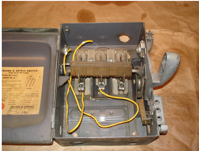
Figure 97: Safety switch before refurbishing.
