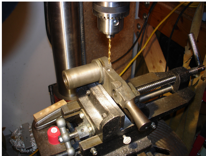
Figure 68: Drilling a hole to remove the plug in the reverse gear casting.
