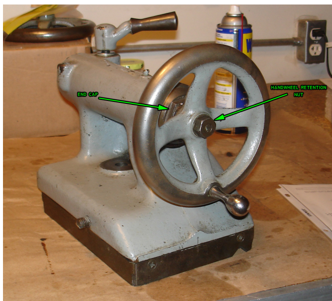
Figure 193: Tailstock showing handwheel parts.
