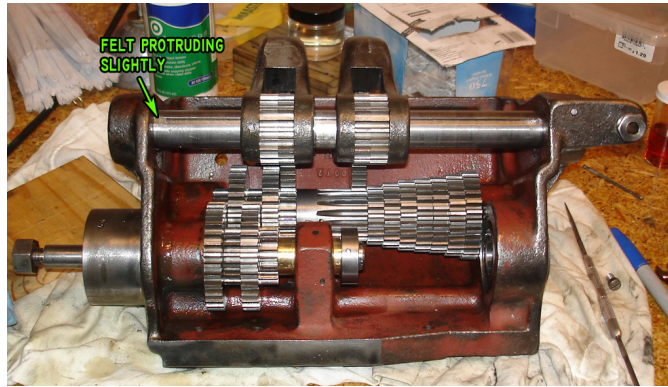
Figure 145: Gearbox showing felt protruding from shift rail.
