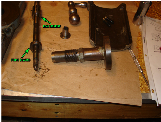
Figure 116: Cross slide parts.
