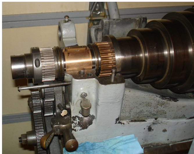
Figure 59: Reinstalled headstock spindle showing rear bearing.
