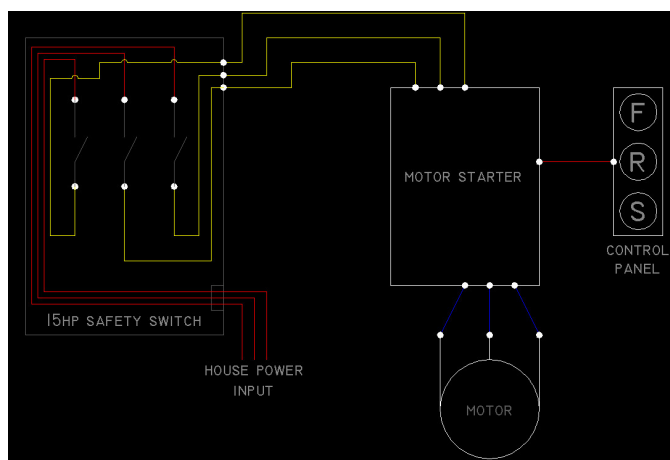
Figure 86: Simple schematic of original wiring.
