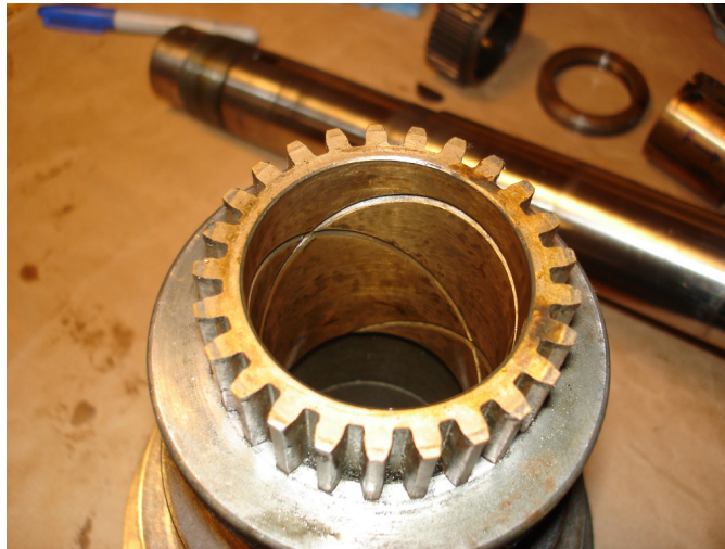
Figure 45: Closeup of rearmost pulley cone bearing.
