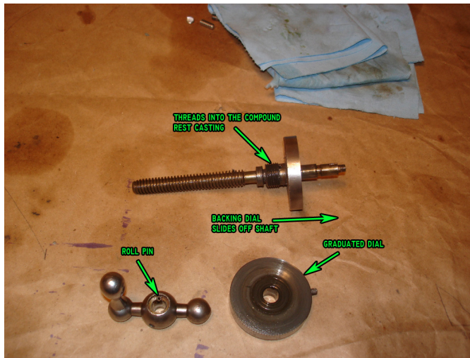
Figure 106: Parts of the compound rest dial.
